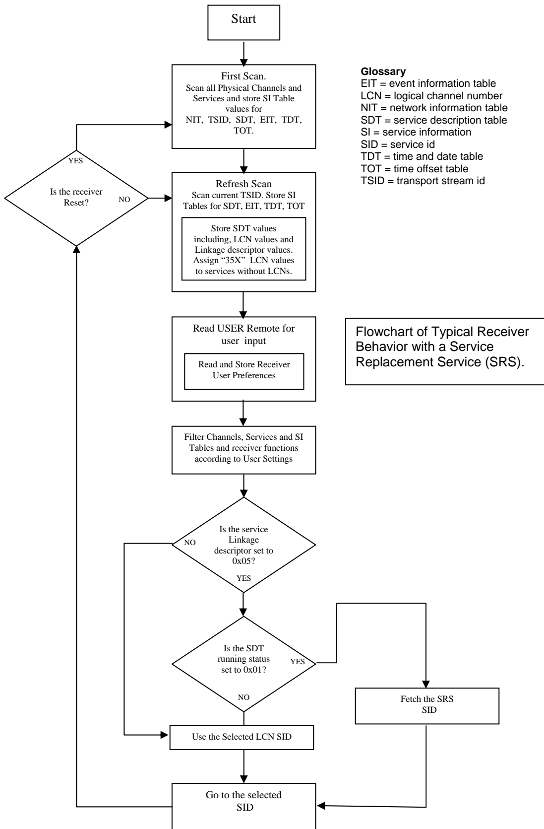
Figure 3: Service Replacement Service – typical receiver behavior.
