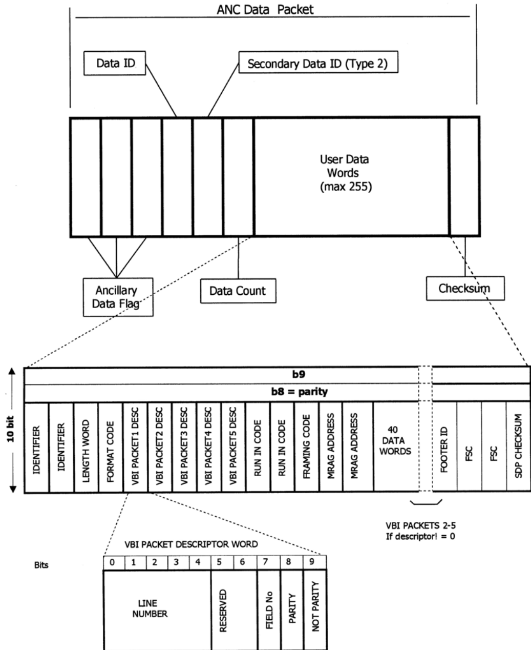
Figure 2: Subtitling Distribution Packet
