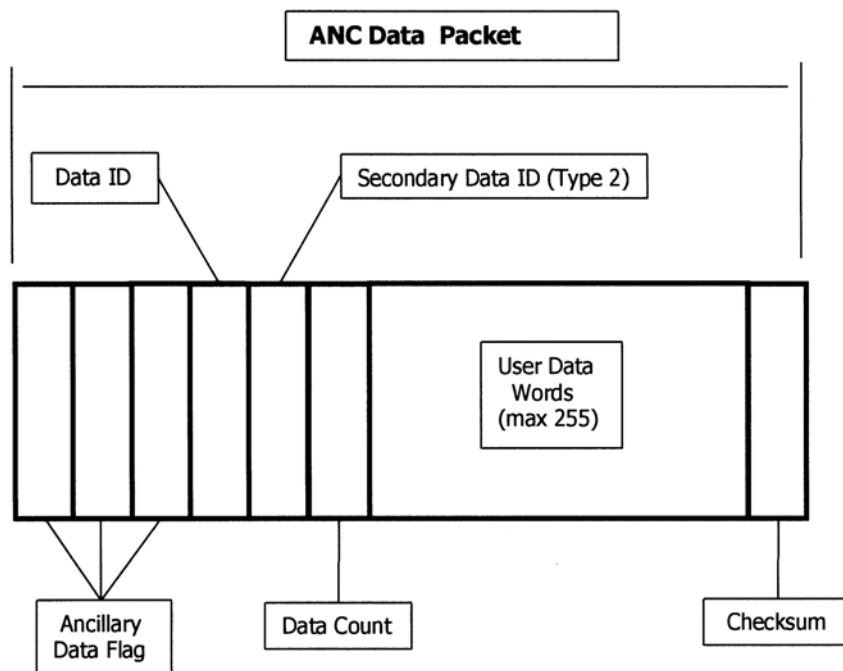
Figure 1: Type 2 Ancillary Data Packet
