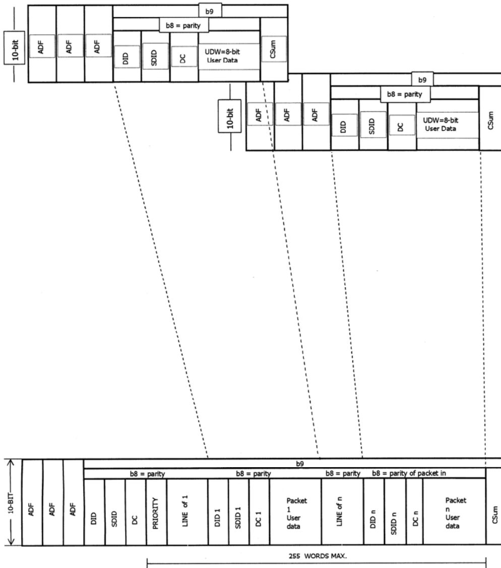
Figure 3: Multipacket Structure
